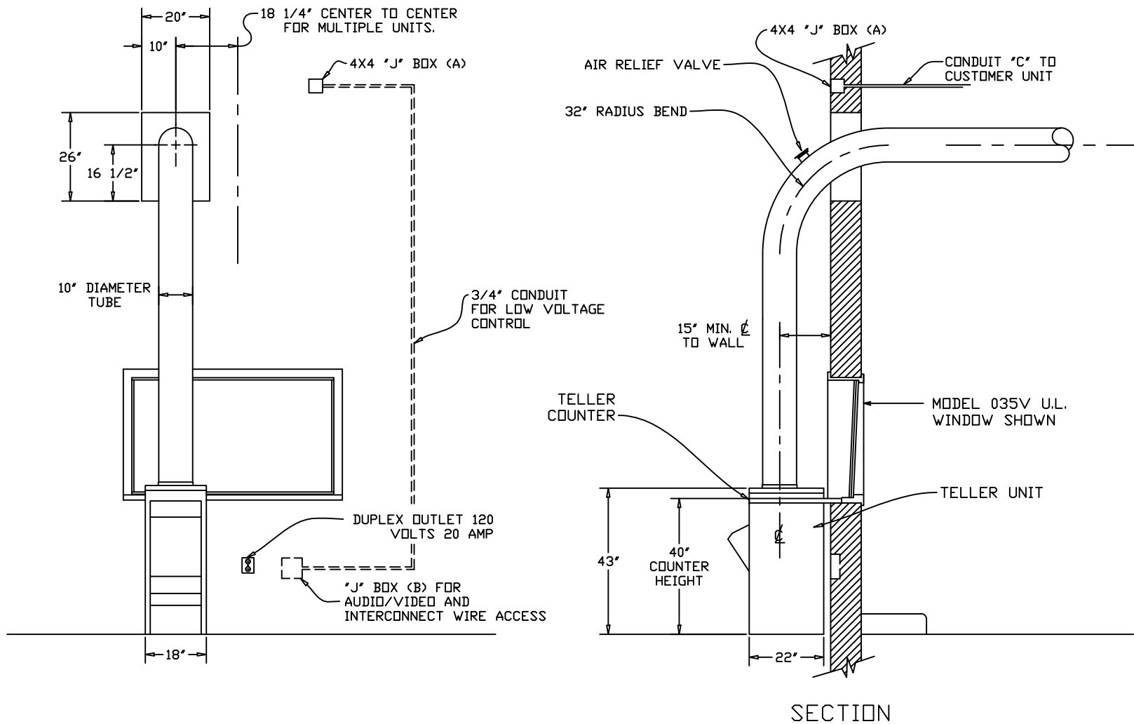
INTERIOR ELEVATION
